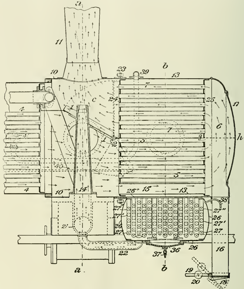
FORNEY'S FEED-WATER HEATER.—LONGITUDINAL SECTION.
